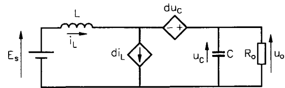
Fig. 5. Boost converter with PWM-switch replaced by the model shown in Fig. 3.
