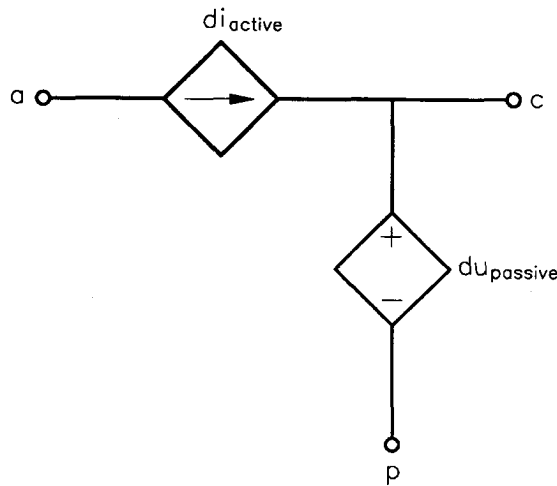
Fig. 8. Generalized PWM-switch model.
