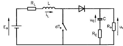
Fig. 6. Boost converter with ESR's.
