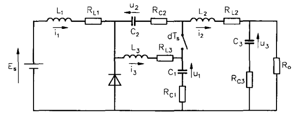
Fig. 9. Topology with separated PWM-switch [4].
