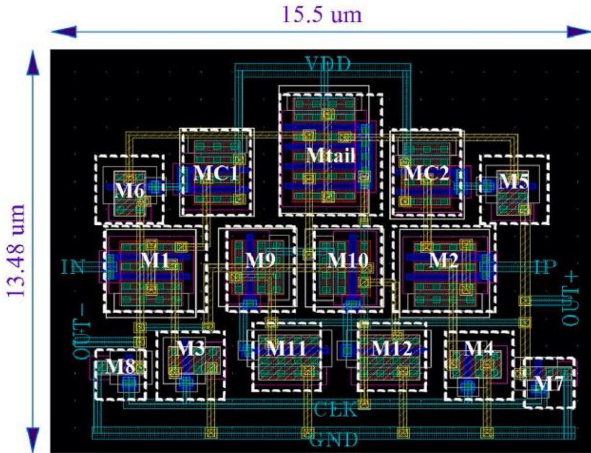
Fig. 12. Layout of the proposed dynamic comparator.
