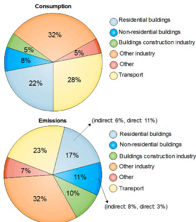
Fig. 1. World's energy consumption and emissions by sector, in 2019 [14,15].
