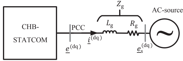
Fig. 3.7 Power system model.
