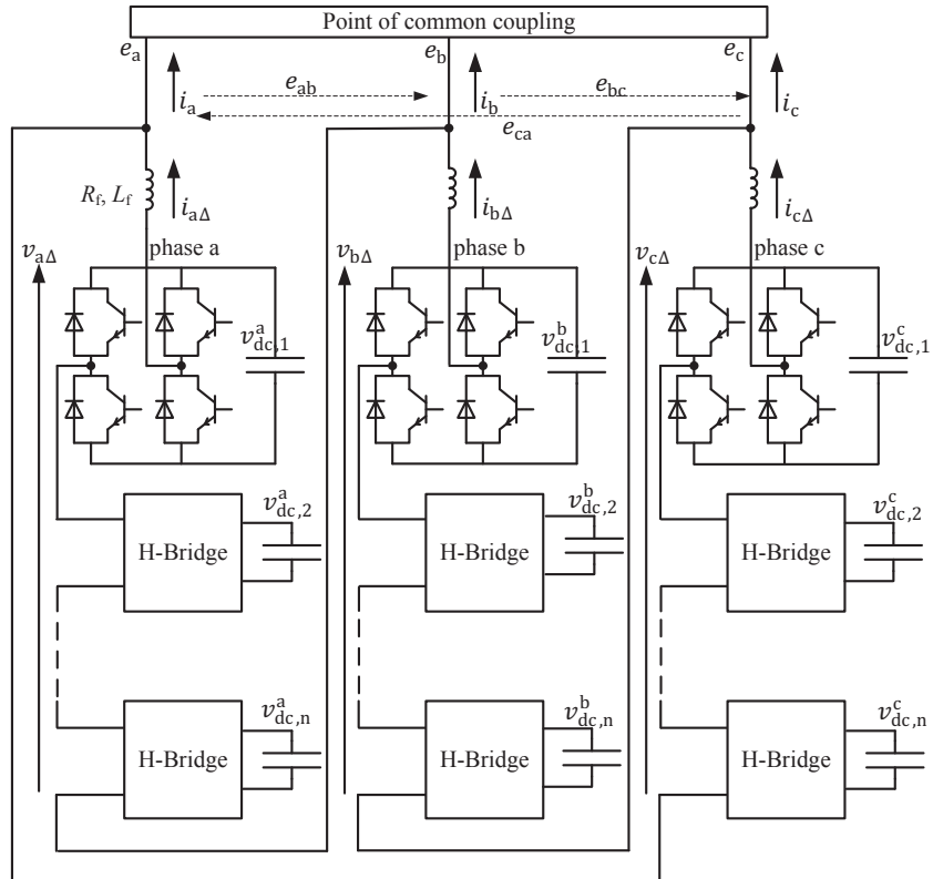
Fig. 3.2 Delta configuration.
