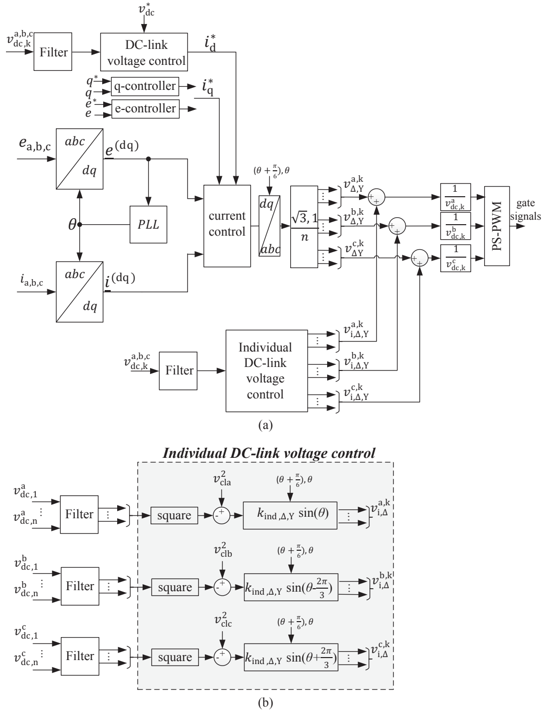
Fig. 4.15 Overall control block diagram CHB-STATCOMs with individual DC-link voltage controller; (a): Overall control; (b): individual DC-link voltage controller.
