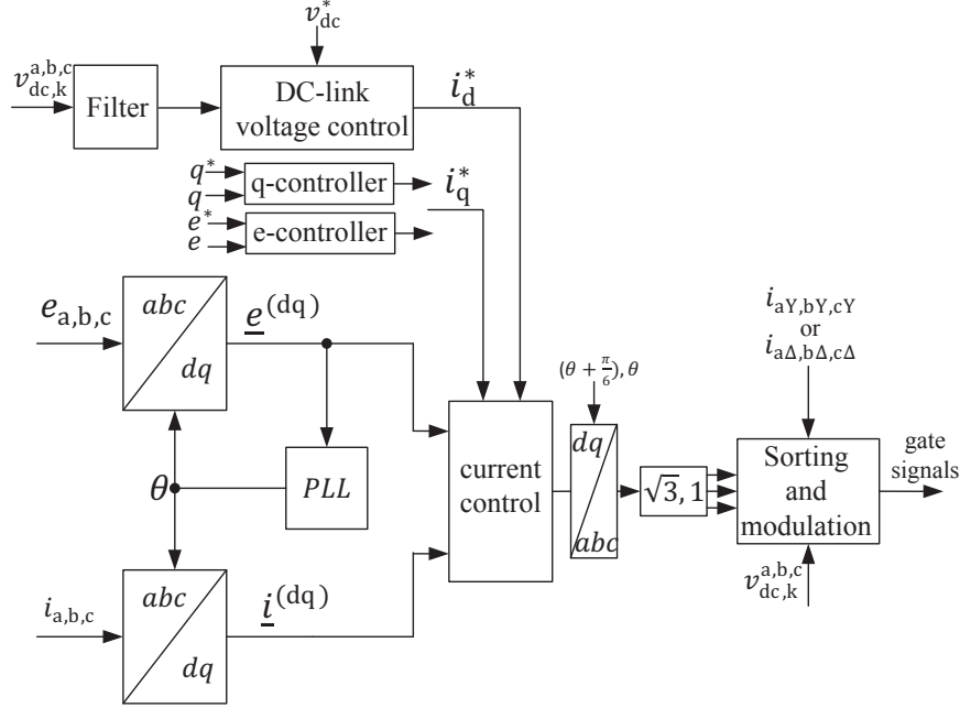
Fig. 4.18 Overall control block diagram of CHB-STATCOM using the sorting approach.
