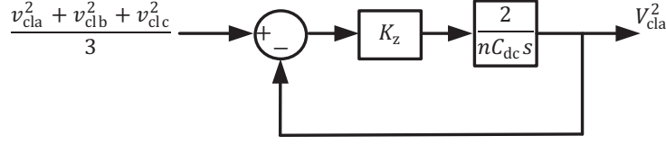
Fig. 5.6 Closed-loop block diagram of the cluster voltage controller.
